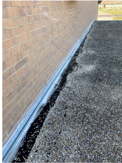
Roof Condition at Wall Flashing
